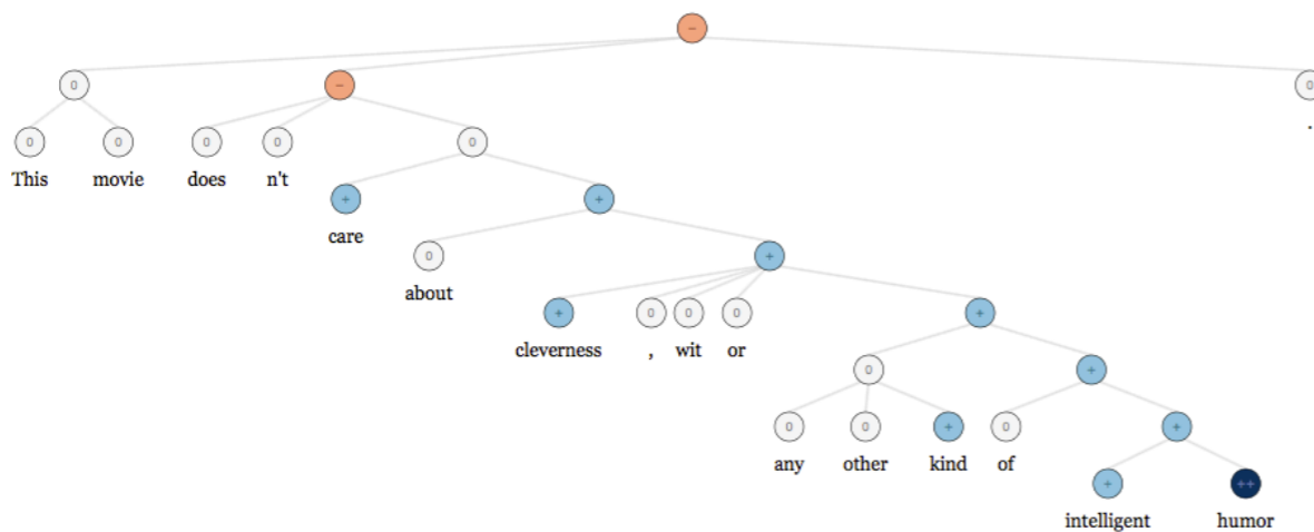
Language Models
